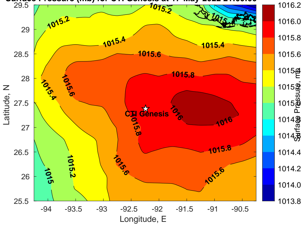
Surface Pressure (mb) for CTI Genesis at 17-May-2022 21:00:00
